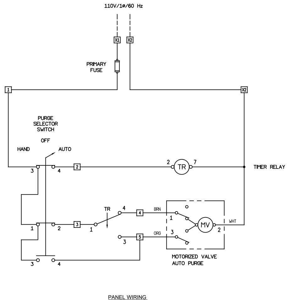
PANEL WIRING
