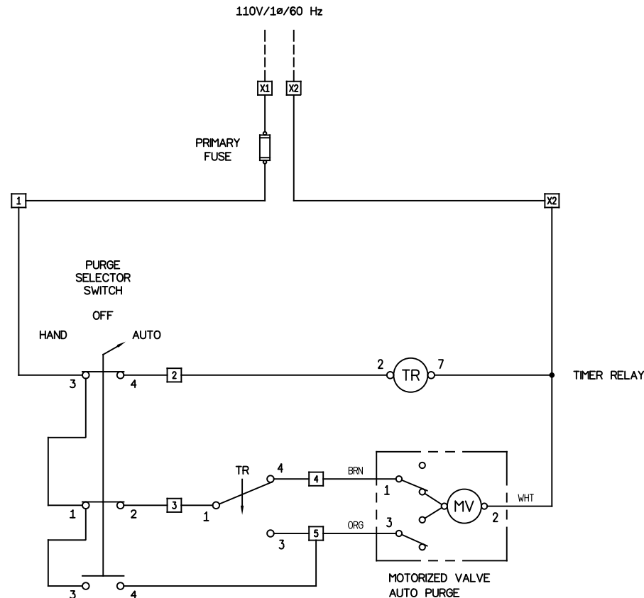
PANEL WIRING
